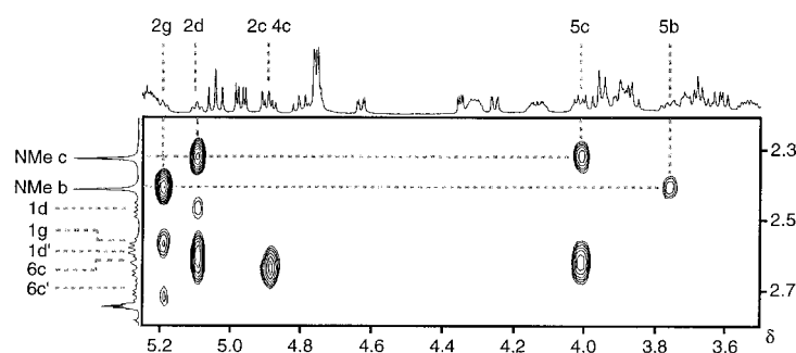
Figure 5. Section from the TROESY spectrum of acetylated dendron 15 (500 MHz, [D_7] DMF), showing crosspeaks to the NMe groups.
