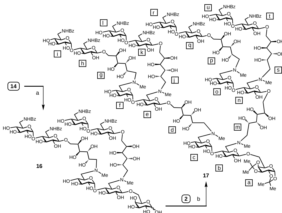
Scheme 5. Reagents: a) \text{TFA}/\text{H}_2\text{O} (9:1) (60%); b) \text{NaCNBH}_3/\text{AcOH}/\text{MeOH} (25%). Monosaccharide residue labels (in squares) for compound 17 relate to ^1\text{H} NMR spectra assignments given in Figure 7 and the Experimental Section
