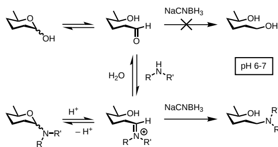
Scheme 1. Reductive amination. The aldehyde function of a reducing sugar reacts with a secondary amine to provide an iminium ion which is selectively reduced by NaCNBH 3 , under neutral conditions to give a tertiary amine. The aldehyde group is not susceptible to reduction by NaCNBH 3 under these conditions.
