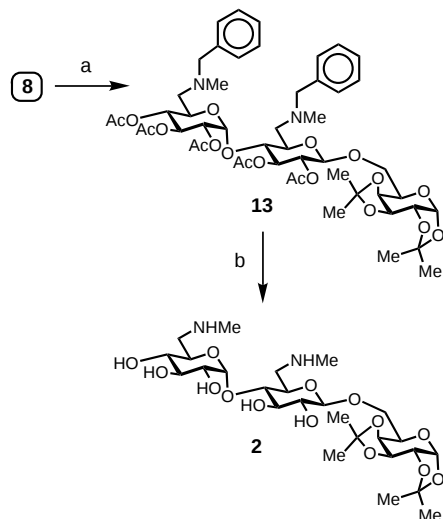
Scheme 3. Reagents: a) 1. MeNHBn/ \Delta , 2. Ac 2 O/C 5 H 5 N (42% over two steps); b) 1. NaOMe/MeOH, 2. H 2 /Pd(OH) 2 on C/MeOH (92% over two steps).
