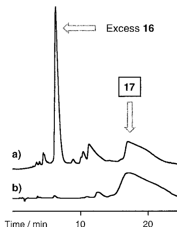
Figure 6. C-18 Reversed phase HPLC analysis (MeOH/ \text{H}_2\text{O} /TFA, 65:35:0.0001 \rightarrow 90:10:0.0001) of a) the reductive amination reaction mixture and b) the 21-mer dendron 17 , following isolation by gel permeation chromatography.
