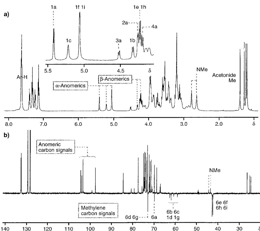
Figure 3. a) ^1\text{H} NMR spectrum (500 MHz, \text{CD}_3\text{OD} ) of dendron 14 with an expansion of the anomeric region inset. b) DEPT-135 spectrum (125 MHz, \text{CD}_3\text{OD} ) of the same compound, showing low intensity signals for nuclei around the branching point of the dendron.
