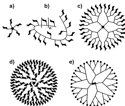
Figure 1. Graphical representation of multivalent neoglycoconjugates: a) glycocluster, b) glycopolymer, c) carbohydrate-coated dendrimer, d) carbohydrate-based dendrimer, and e) carbohydrate-centered dendrimer.
