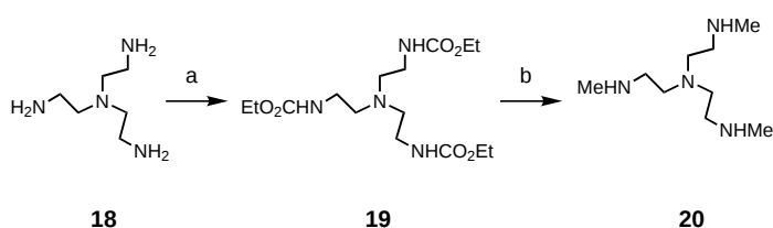
Scheme 6. Reagents: a) \text{ClCO}_2\text{Et}/\text{C}_6\text{H}_6/\text{H}_2\text{O}/\text{KOH} (40%); b) \text{LiAlH}_4/\text{THF} (56%).
