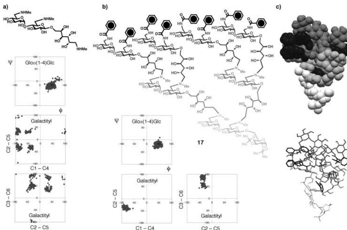
Figure 9. Plots of torsion angles, sampled during MD simulations, for the Glc \alpha (1 \rightarrow 4)Glc glycosidic linkage ( \phi vs. \psi ) and the carbon backbone of the galactityl residue (C1–C4 vs. C2–C5 and C2–C5 vs. C3–C6) in a) an isolated trisaccharide repeat unit and b) representative examples from the second-generation dendron 17 . The MD simulations were conducted for a) 1 ns and b) 5 ns at 300 K as described in the Experimental section. c) Space-filling and polytube representations of the second-generation dendron 17 , highlighting the constituent trisaccharide residues in light grey through to dark grey and the peripheral benzamide groups in black.
