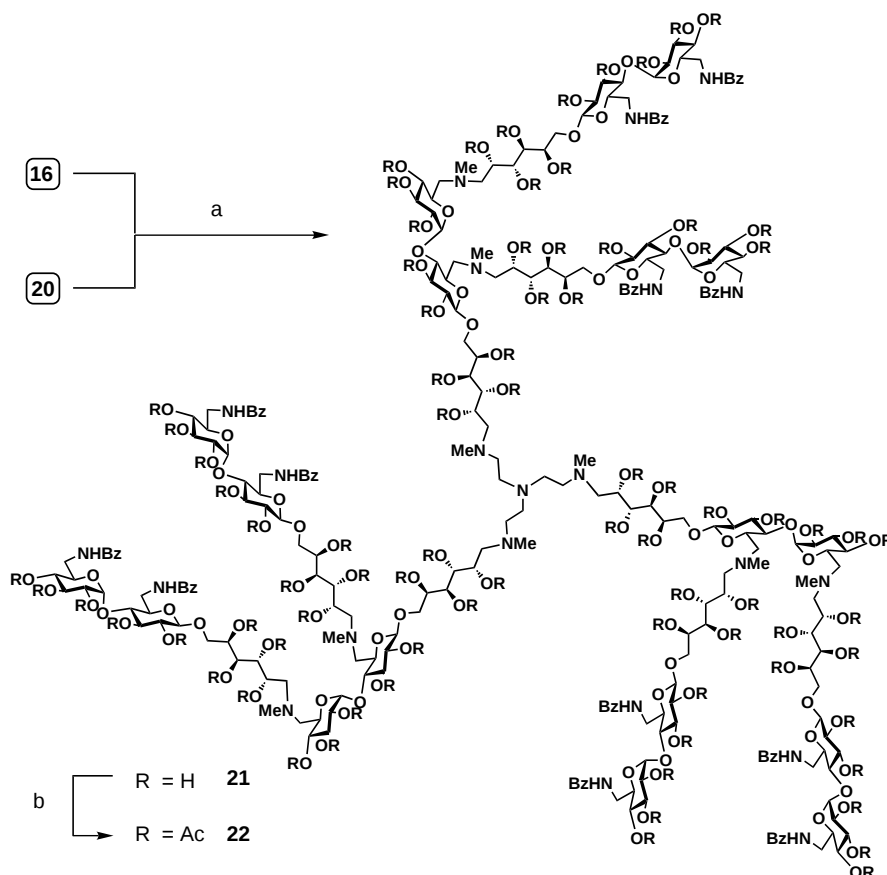
Scheme 7. Reagents: a) \text{NaCNBH}_3/\text{AcOH}/\text{MeOH} (54%); b) \text{Ac}_2\text{O}/\text{C}_5\text{H}_5\text{N}/\text{DMAP} (50%).
