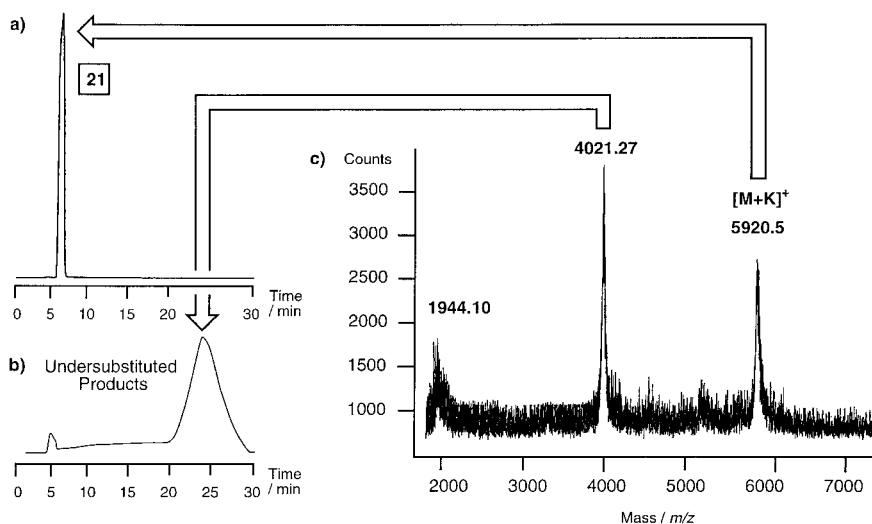
Figure 8. GPC traces of a) first-generation dendrimer 21 , b) undersubstituted products of the reductive amination reaction, and c) a MALDI-TOF mass spectrum of the product mixture isolated from the reaction.
