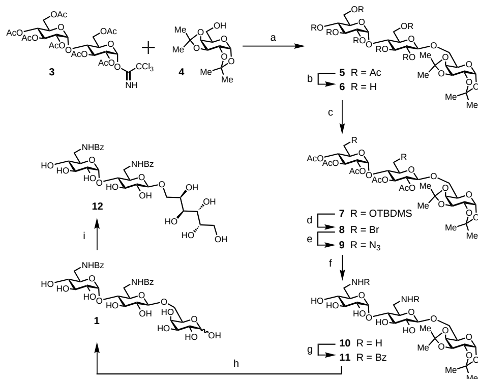
Scheme 2. Reagents: a) \text{TMSOTf}/\text{CH}_2\text{Cl}_2/4 \text{ \AA MS} (81%); b) \text{NaOMe}/\text{MeOH} (97%); c) 1. \text{TBDMSCl}/\text{C}_5\text{H}_5\text{N} , 2. \text{Ac}_2\text{O}/\text{C}_5\text{H}_5\text{N} (75% over two steps); d) \text{Br}_2/\text{PPh}_3/\text{CH}_2\text{Cl}_2 (95%); e) \text{NaN}_3/\text{DMF} (95%); f) 1. \text{NaOMe}/\text{MeOH} , 2. \text{N}_2\text{H}_4/\text{Pd}(\text{OH})_2 on \text{C}/\text{MeOH} (93% over two steps); g) 1. \text{BzCl}/\text{C}_5\text{H}_5\text{N} , 2. \text{NaOMe}/\text{MeOH} (80% over two steps); h) \text{TFA}/\text{H}_2\text{O} (9:1) (80%); i) \text{NaBH}_4/\text{MeOH} (87%).
