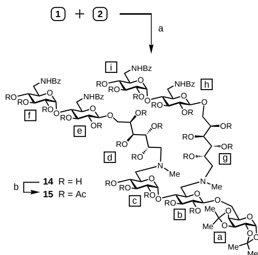
Scheme 4. Reagents: a) NaCNBH 3 /AcOH/MeOH (78%); b) Ac 2 O/C 5 H 5 N (86%). Monosaccharide residue labels (in squares) for compound 14 relate to 1 H NMR spectra assignments given in Figures 3, 4, and 5 and in the Experimental Section.
