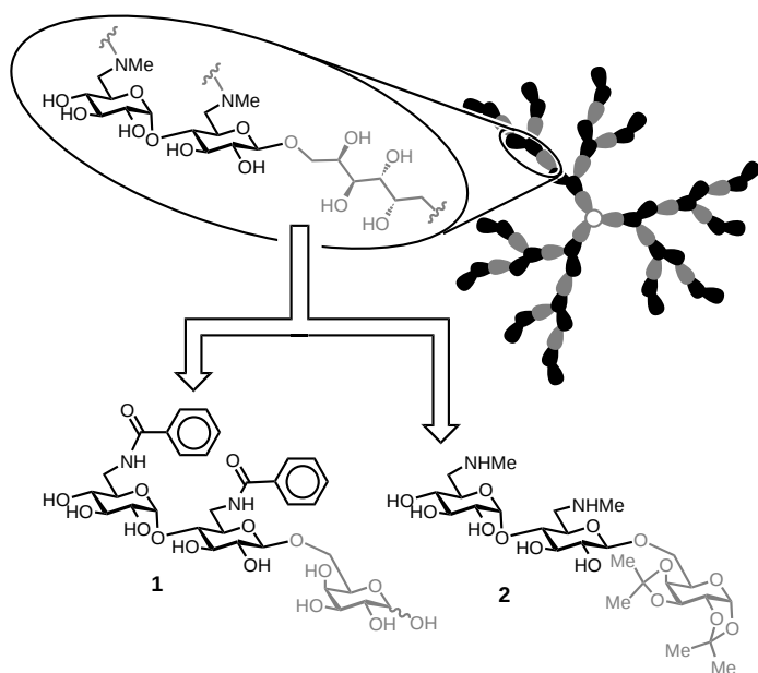
Figure 2. Retrosynthetic analysis of an oligosaccharide-based glycodendrimer with a maltosylgalactosyl trisaccharide repeating unit. The outer portion of the dendrimer is derived from the benzamide-protected reducing sugar 1 , following reductive amination with the diamine 2 , which forms the internal branching units of the dendrimer.
