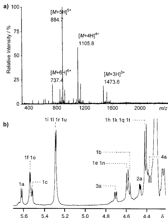
Figure 7. Characterization of the second-generation dendron 17 . a) Electrospray mass spectrum and b) partial ^1\text{H} NMR spectrum (500 MHz, \text{D}_2\text{O} ) showing the anomeric region.
