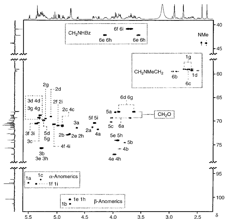
Figure 4. HMQC and DEPT-135 spectra of acetylated dendron 15 (500 MHz, [\text{D}_7]\text{DMF} ), indicating the locations of the anomeric and methylene signals.
